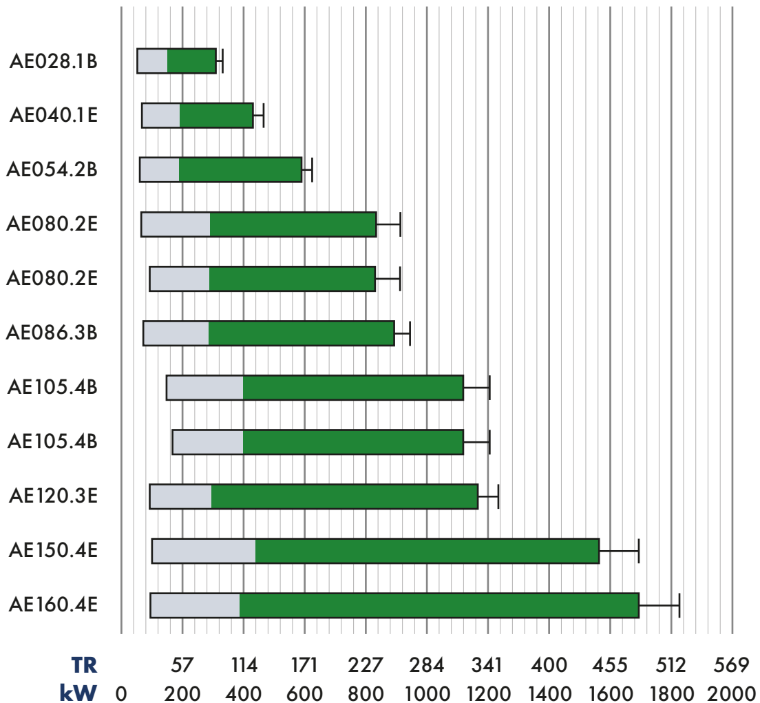
Cooling Capacity TR (kW)
