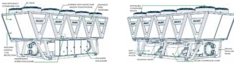
Side and front views of a Smardt T-Class AE Design Series chiller
